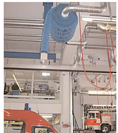
Exhaust Hose Reel 865 in the Vehicle maintenance shop
